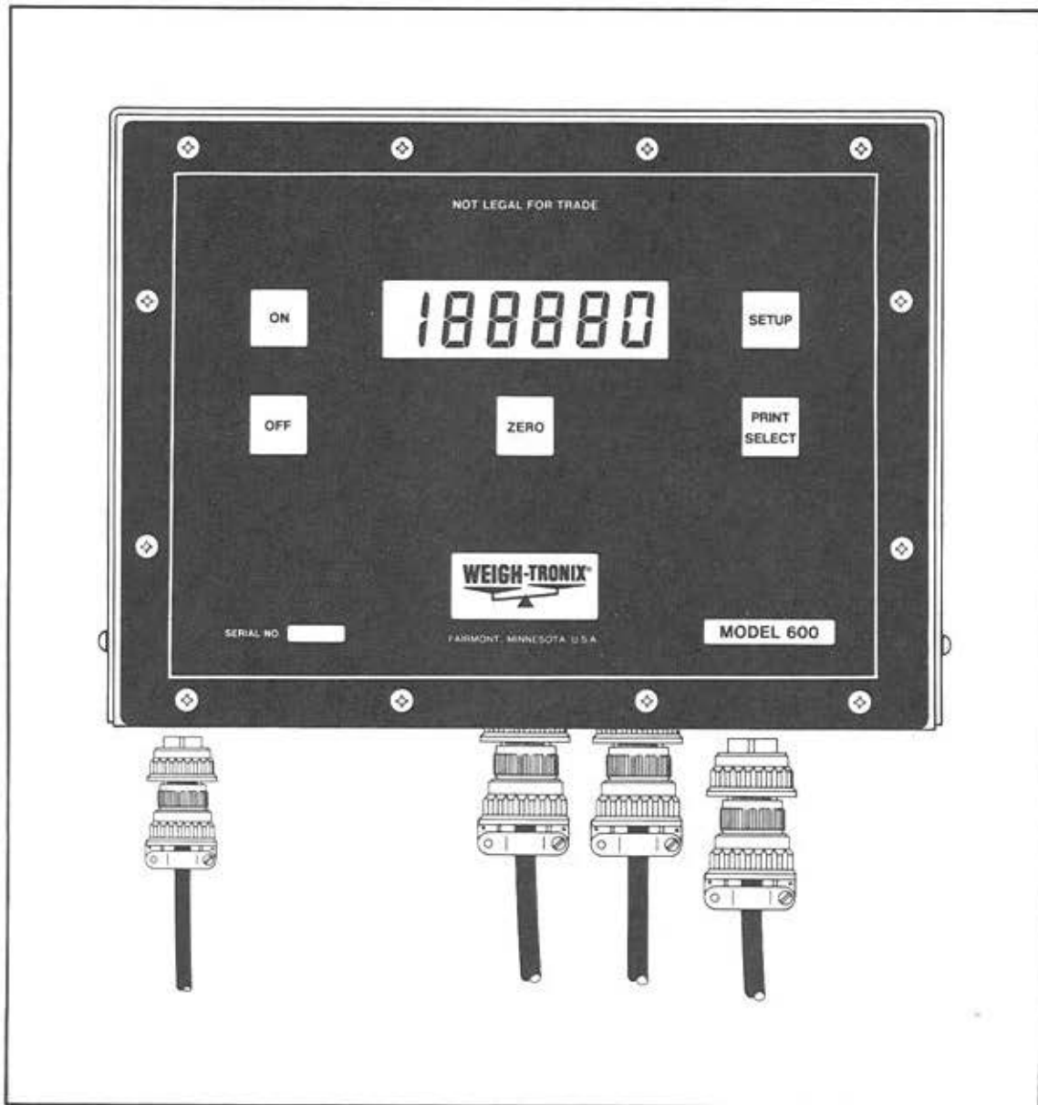
Figure 1: Front Panel of Model 600 Farm Indicator
